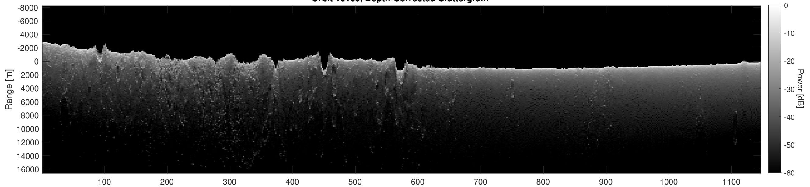
Orbit 10169, Depth-Corrected Cluttergram
