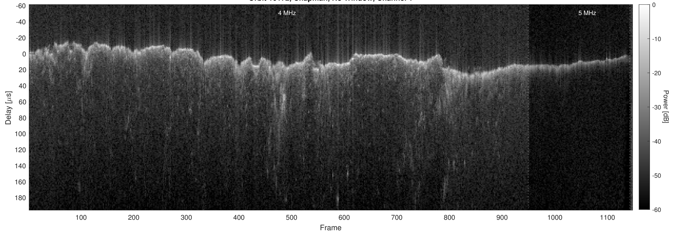
Orbit 10172, Chapman, No Window, Channel 2
