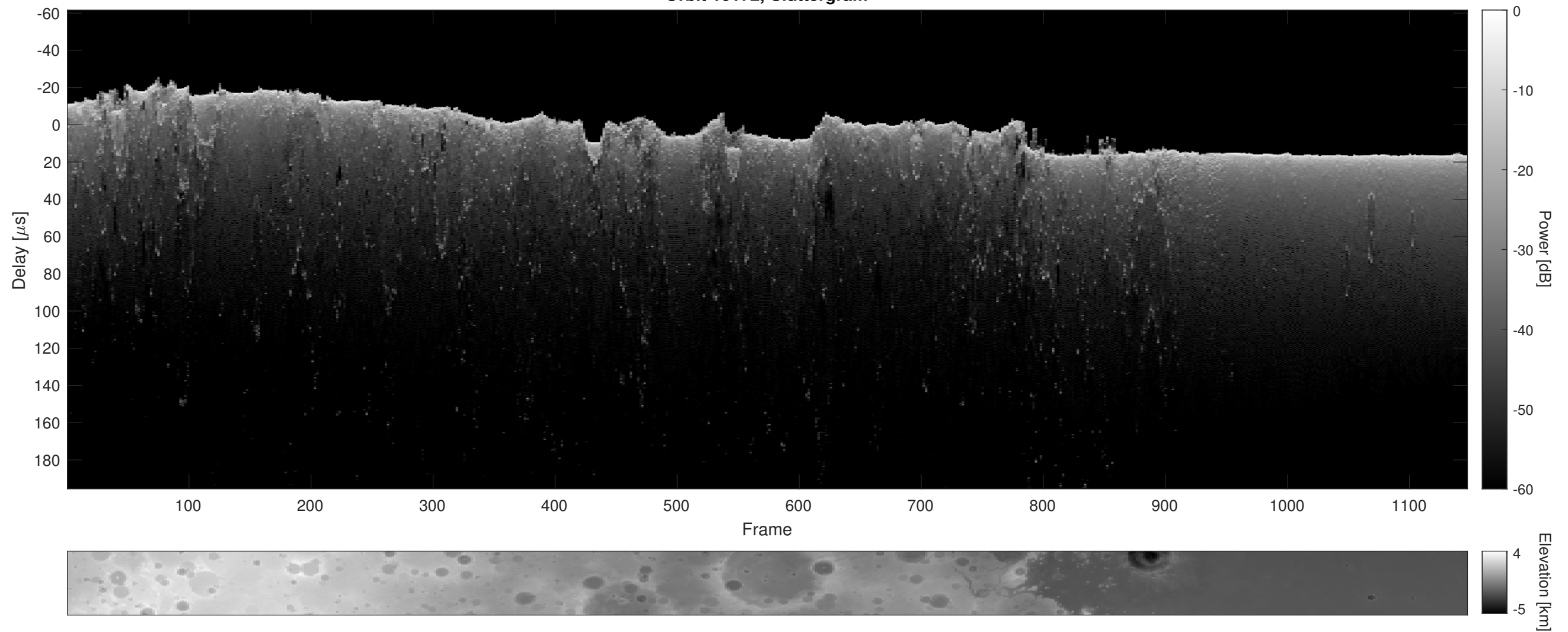
Orbit 10172, Cluttergram
