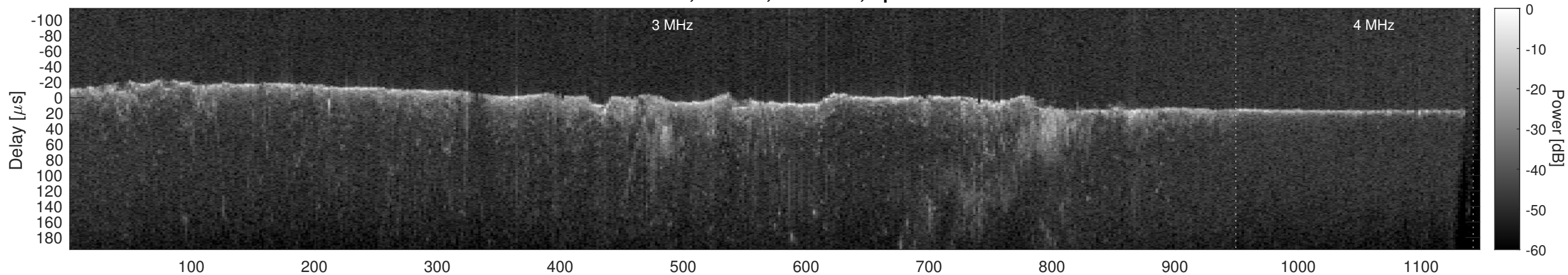
Orbit 10172, Cluttergram
