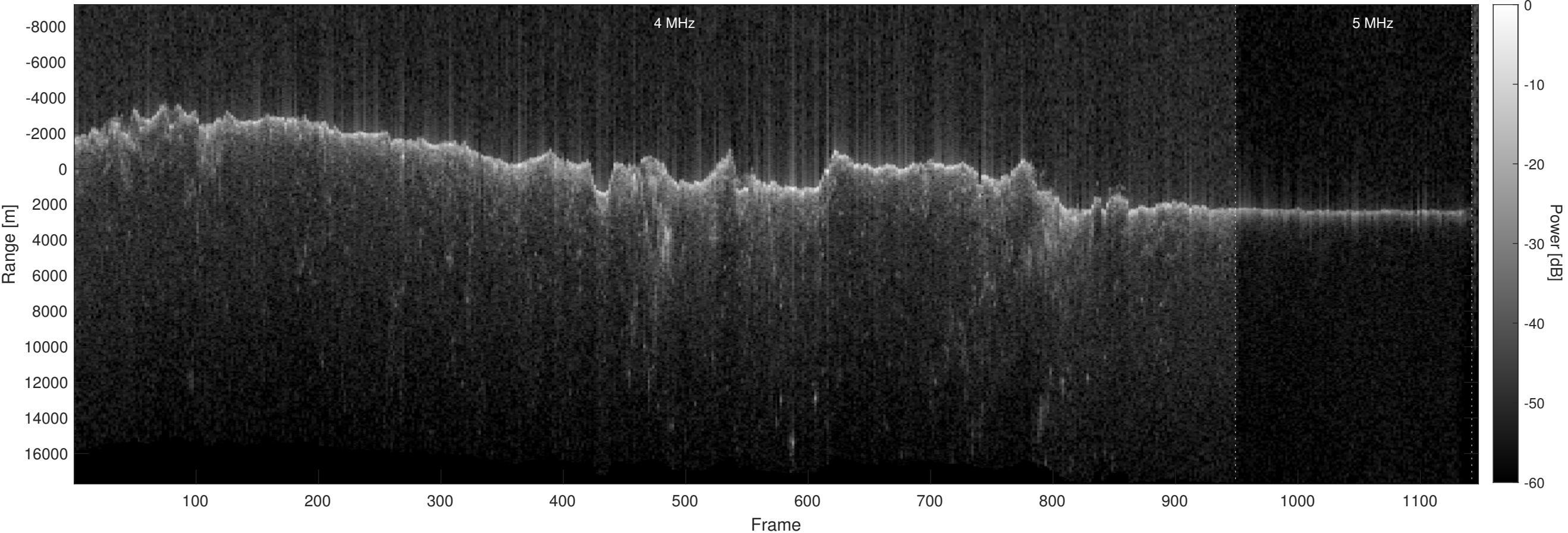
Orbit 10172, Optimized, No Window, Depth-Corrected, Channel 2
