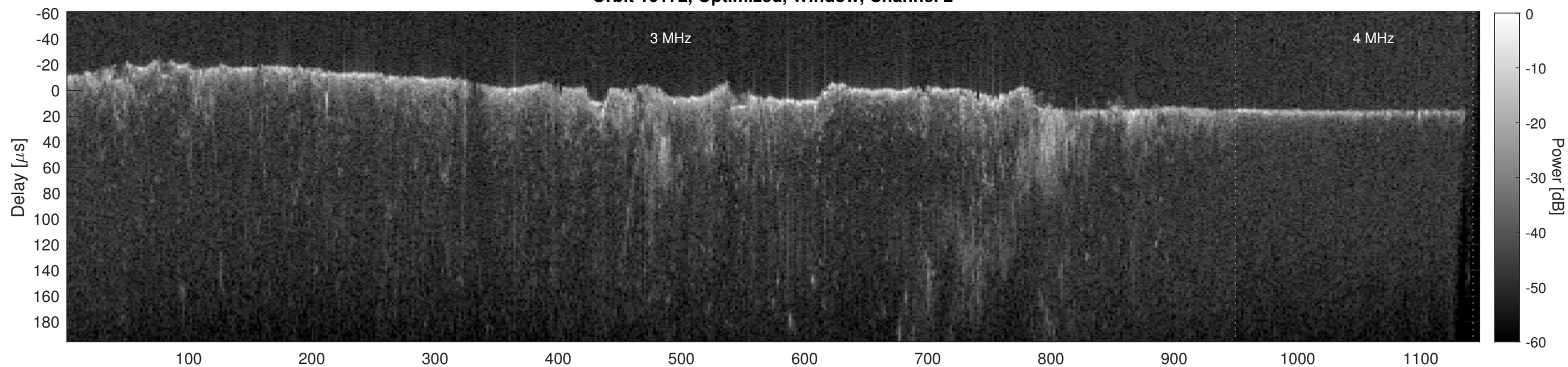
Orbit 10172, Cluttergram
