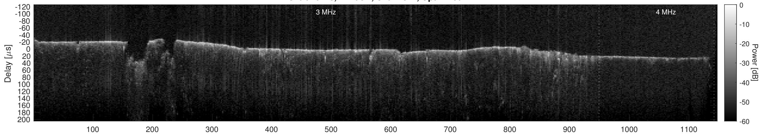
Orbit 10173, Cluttergram
