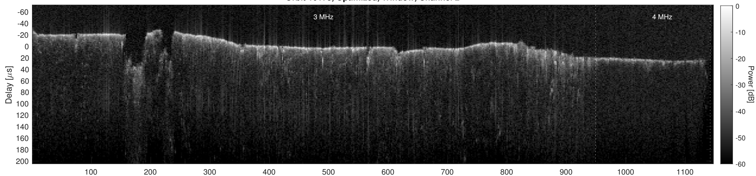
Orbit 10173, Cluttergram
