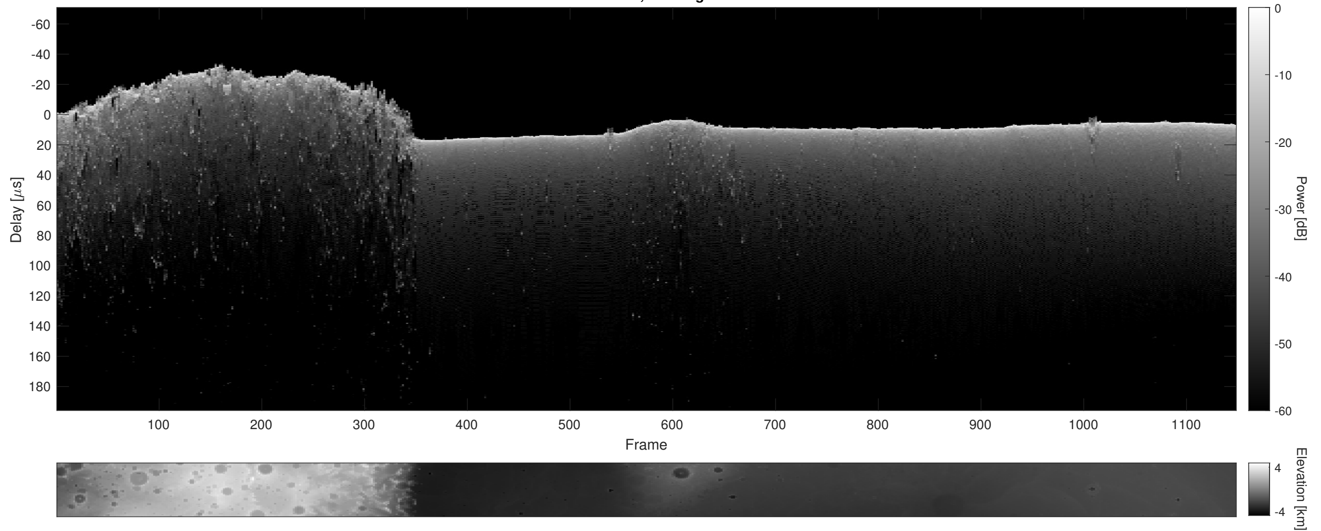
Orbit 10175, Cluttergram
