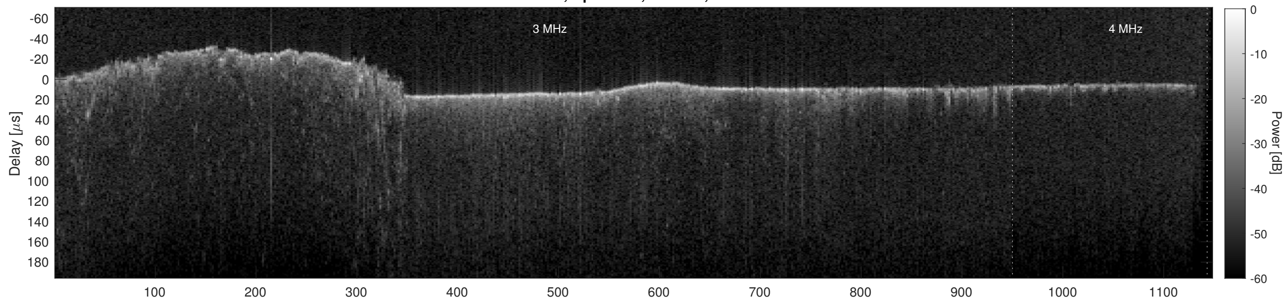
Orbit 10175, Cluttergram
