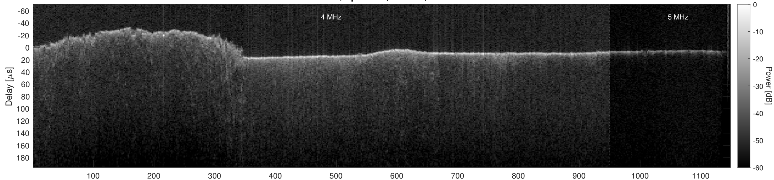
Orbit 10175, Optimized, Window, Channel 2
