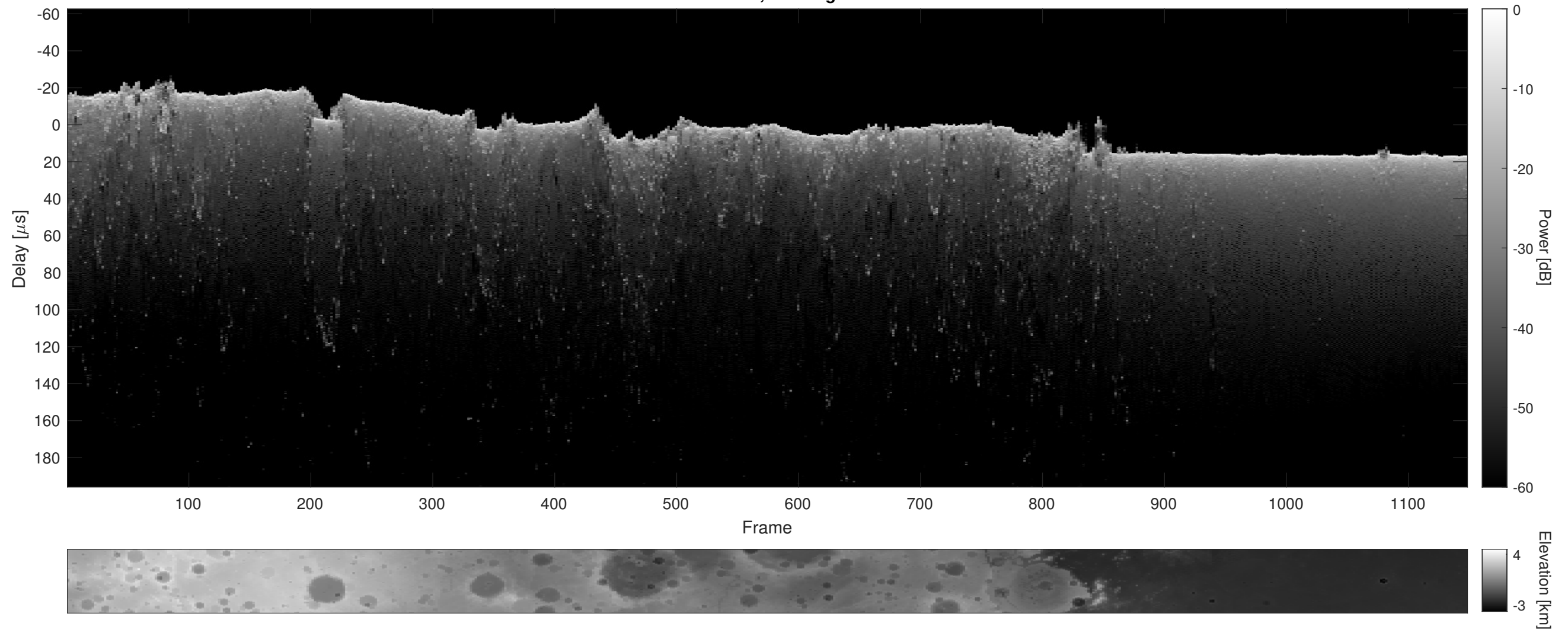
Orbit 10179, Cluttergram
