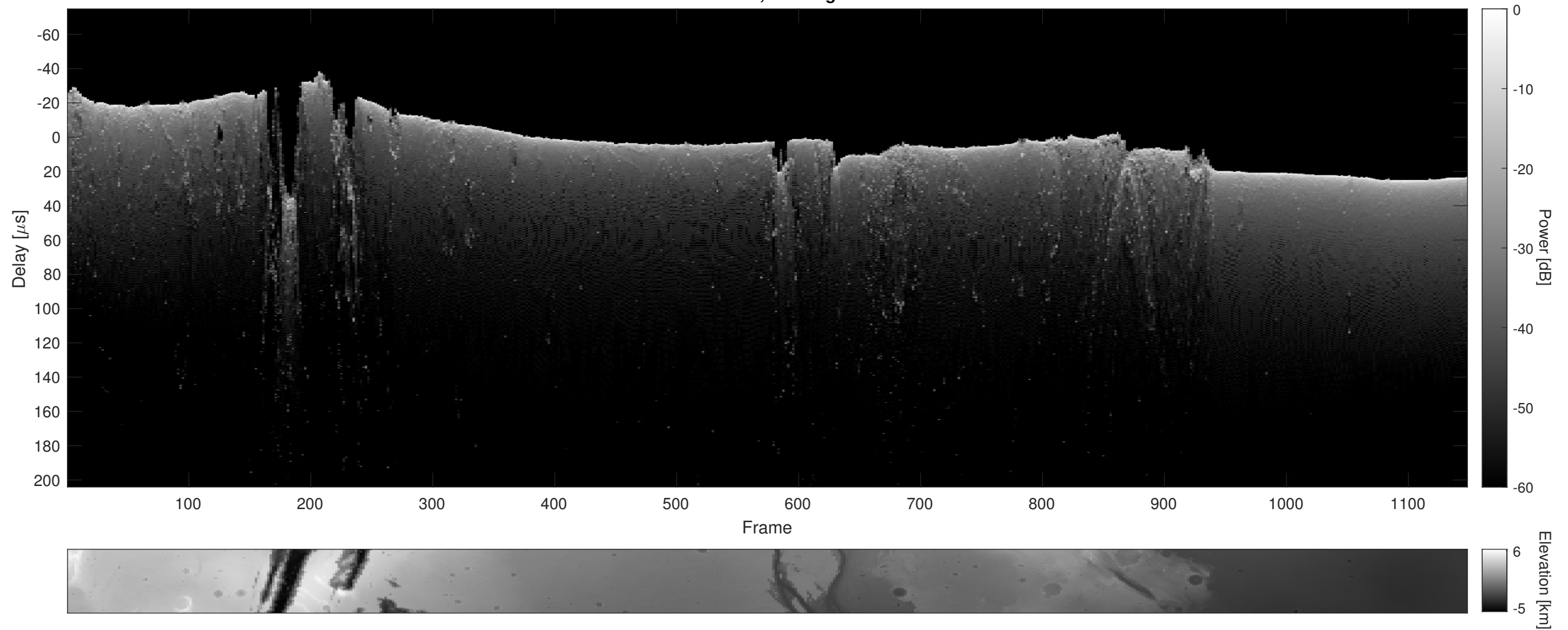
Orbit 10180, Cluttergram
