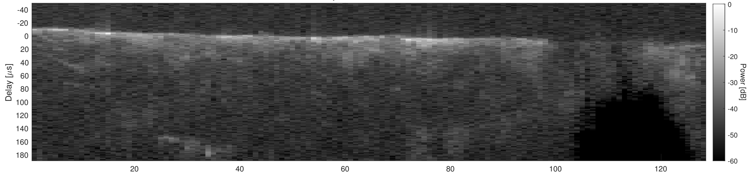
Orbit 10181, Cluttergram
