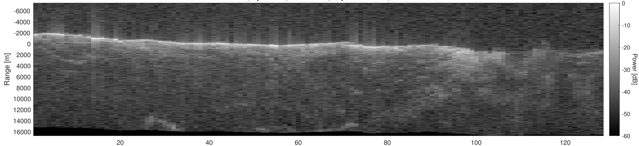
Orbit 10181, Optimized, No Window, Depth-Corrected, Channel 2
