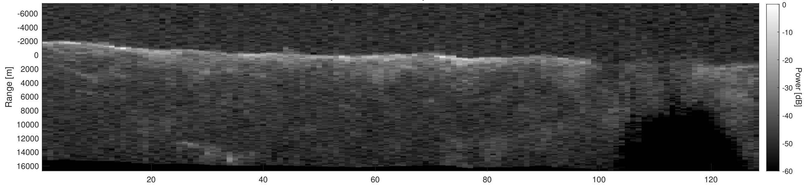
Orbit 10181, Depth-Corrected Cluttergram
