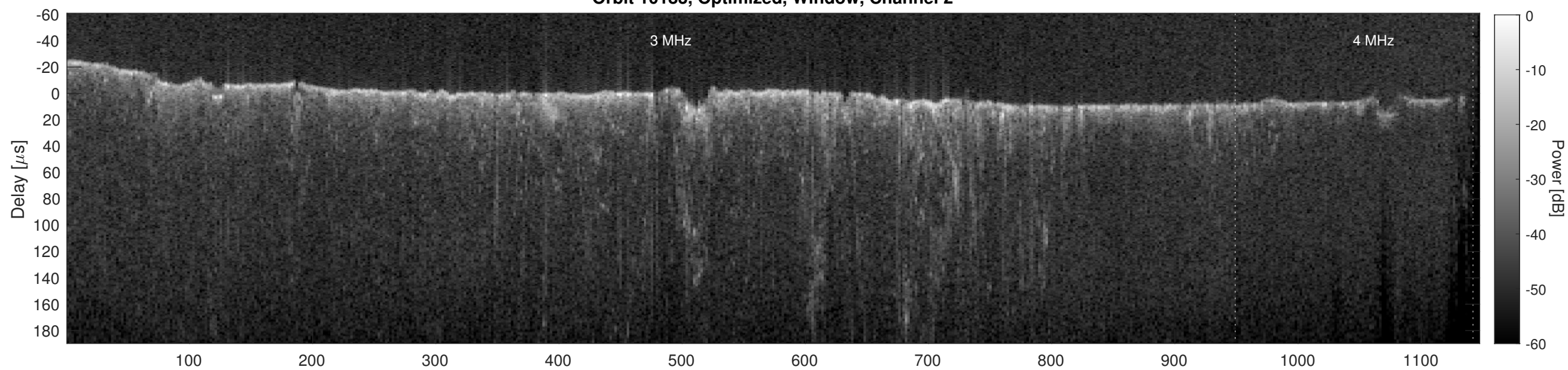
Orbit 10183, Cluttergram
