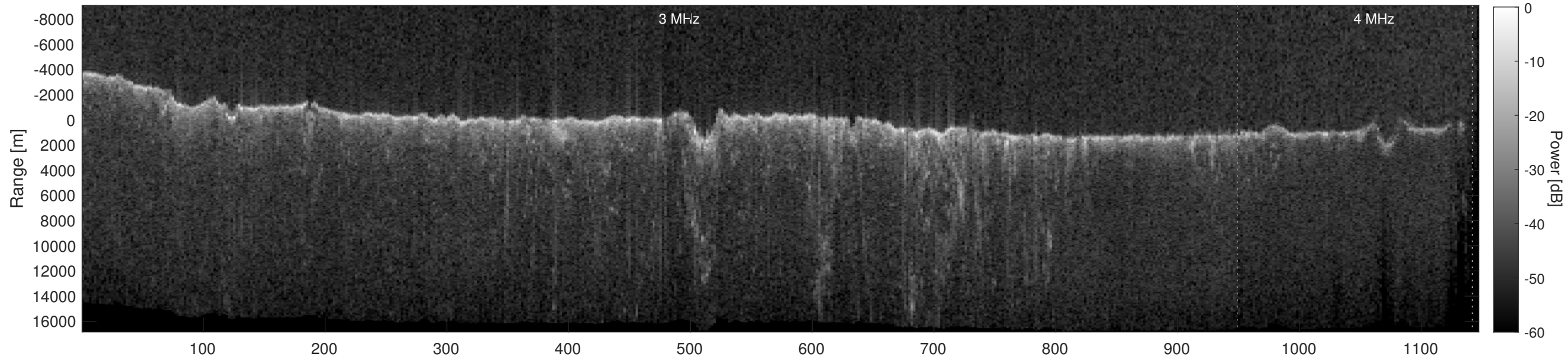
Orbit 10183, Depth-Corrected Cluttergram
