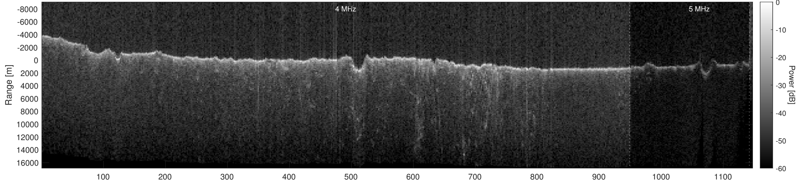
Orbit 10183, Optimized, Window, Depth-Corrected, Channel 2
