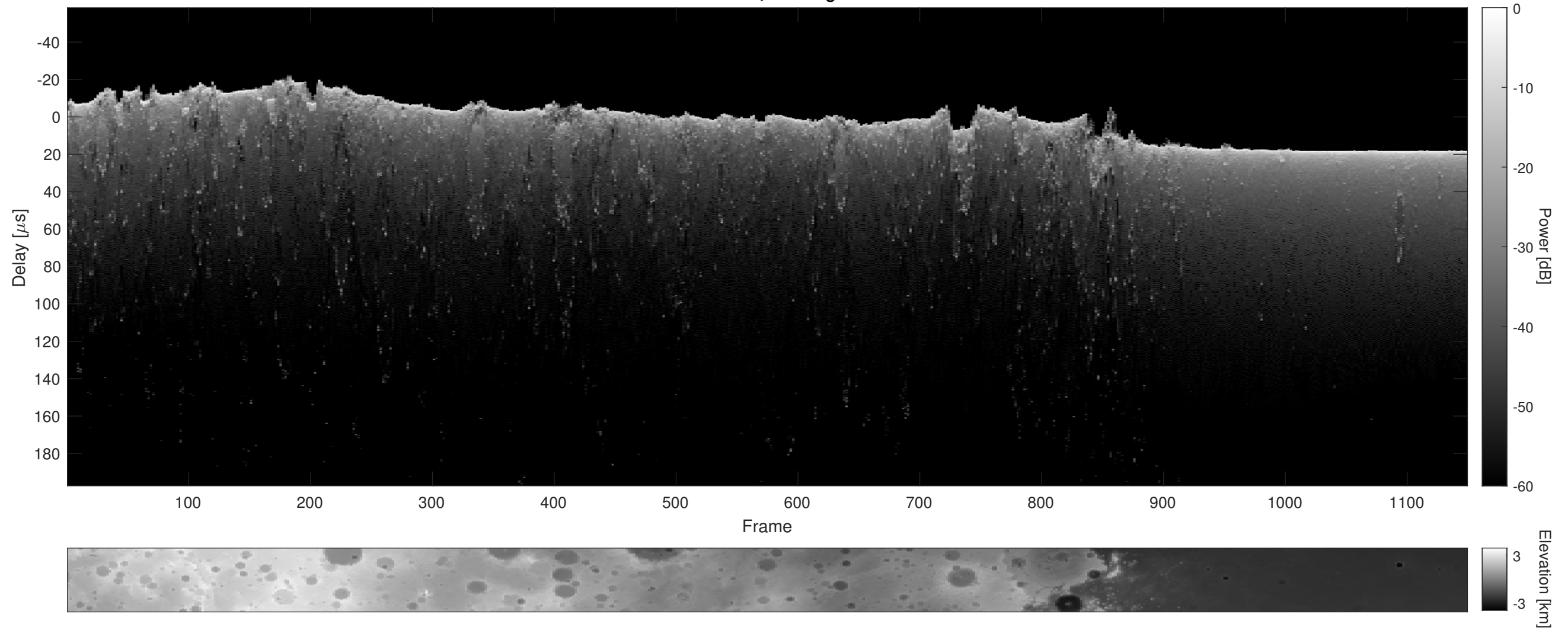
Orbit 10186, Cluttergram
