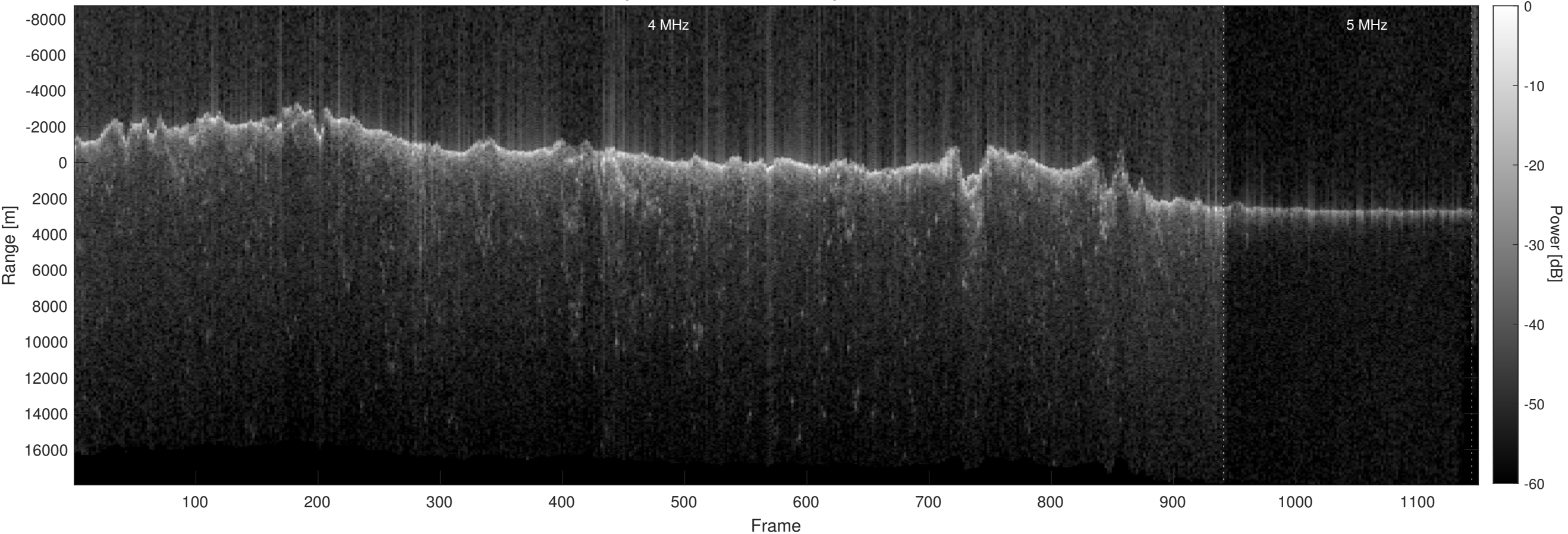
Orbit 10186, Optimized, No Window, Depth-Corrected, Channel 2
