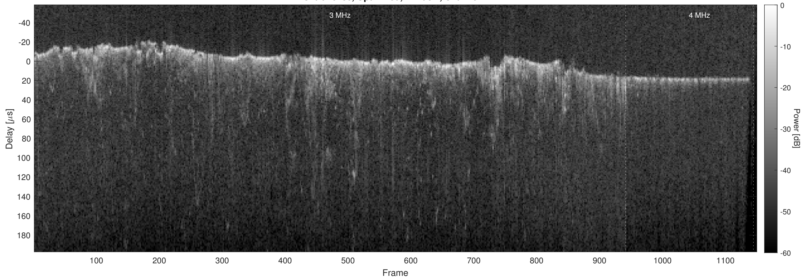
Orbit 10186, Optimized, Window, Channel 2
