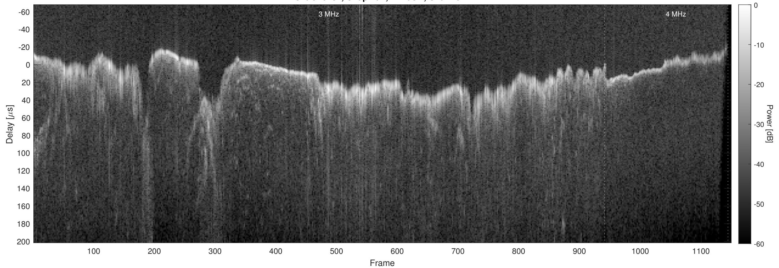
Orbit 10187, Chapman, Window, Channel 2
