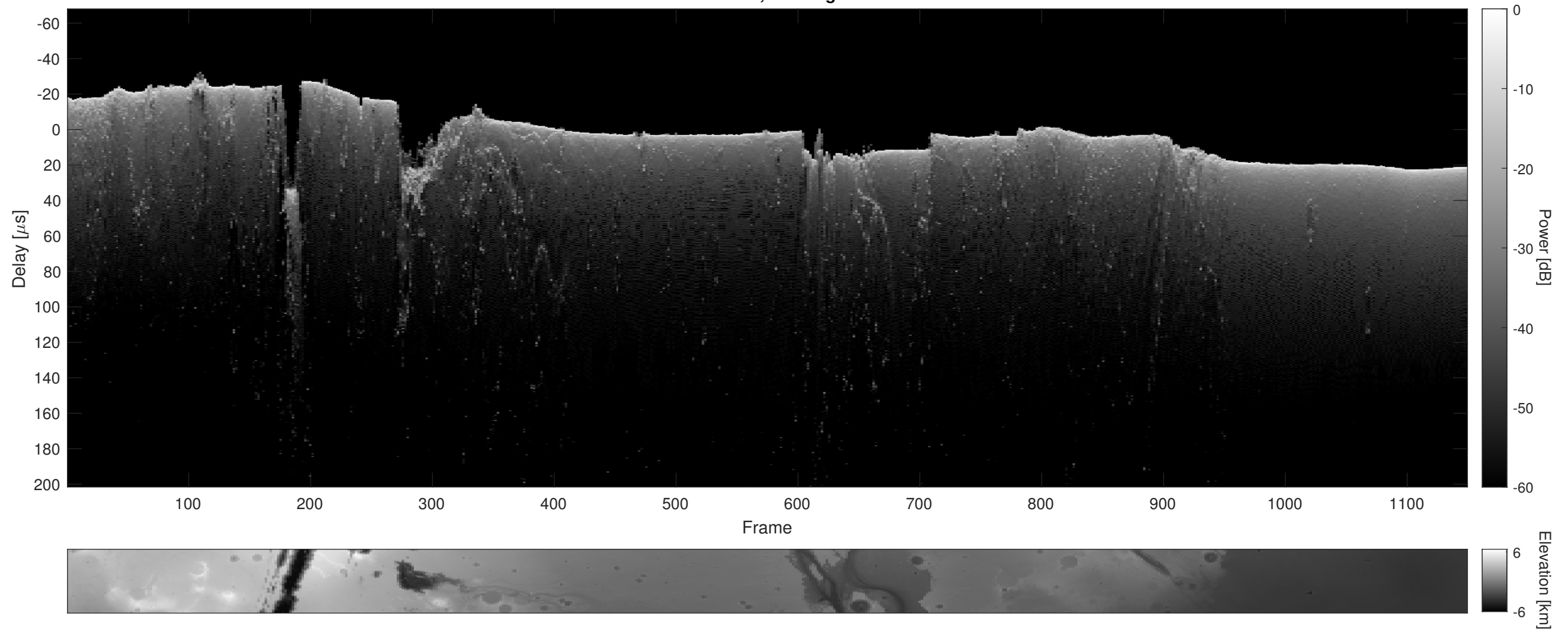
Orbit 10187, Cluttergram
