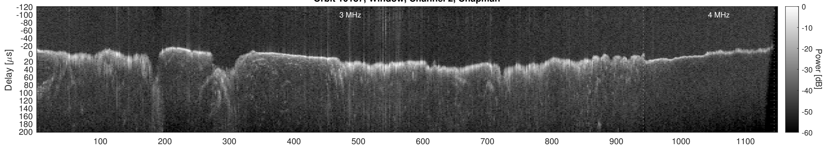
Orbit 10187, Window, Channel 2, Optimized
