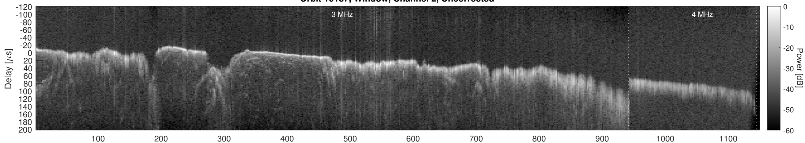
Orbit 10187, Window, Channel 2, Chapman
