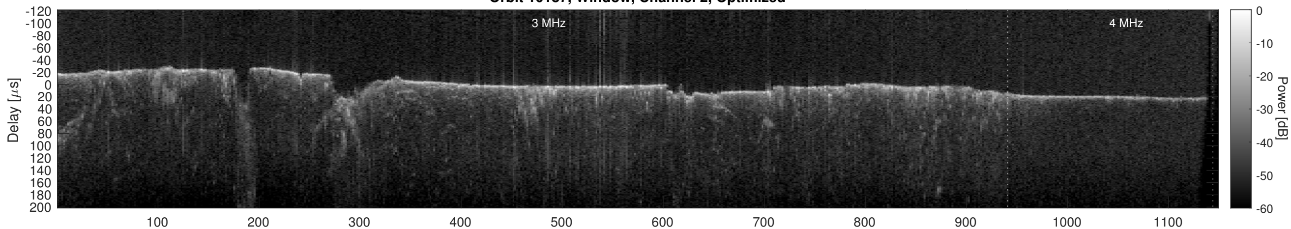
Orbit 10187, Cluttergram
