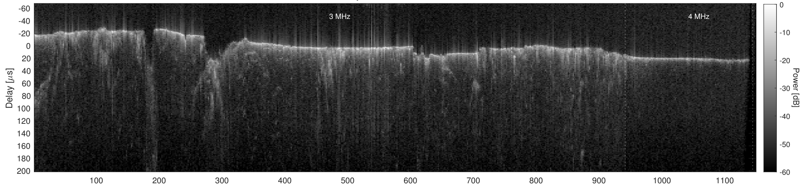
Orbit 10187, Cluttergram
