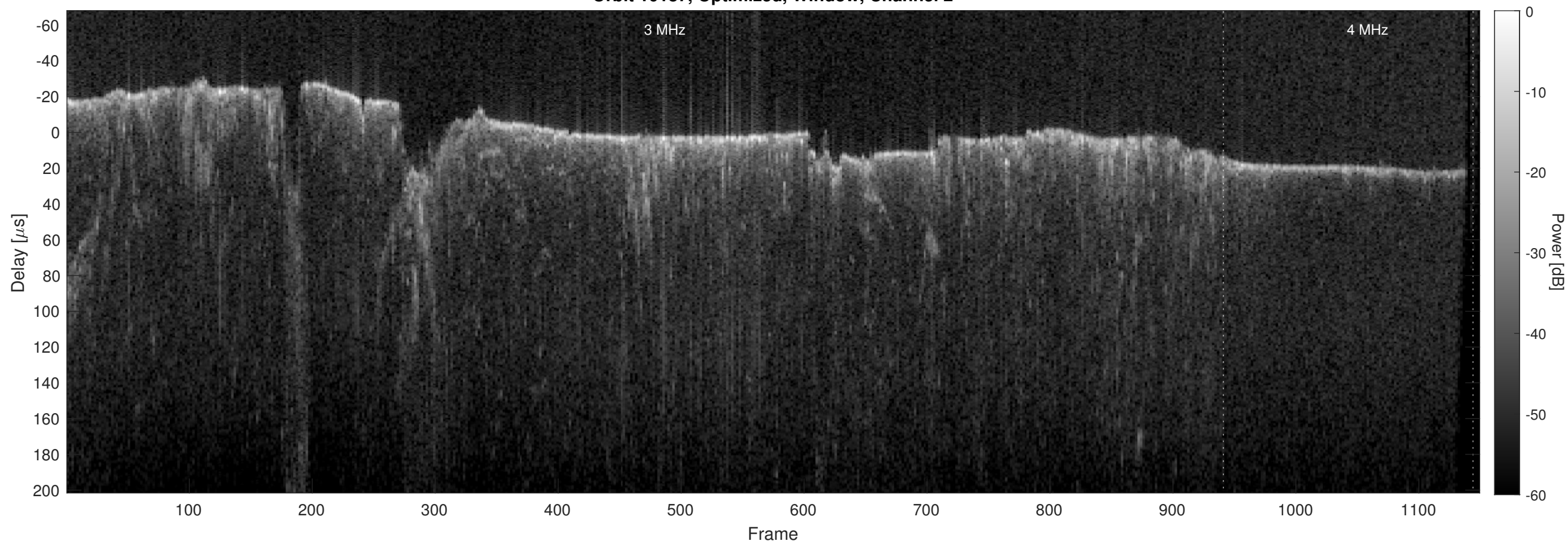
Orbit 10187, Optimized, Window, Channel 2
