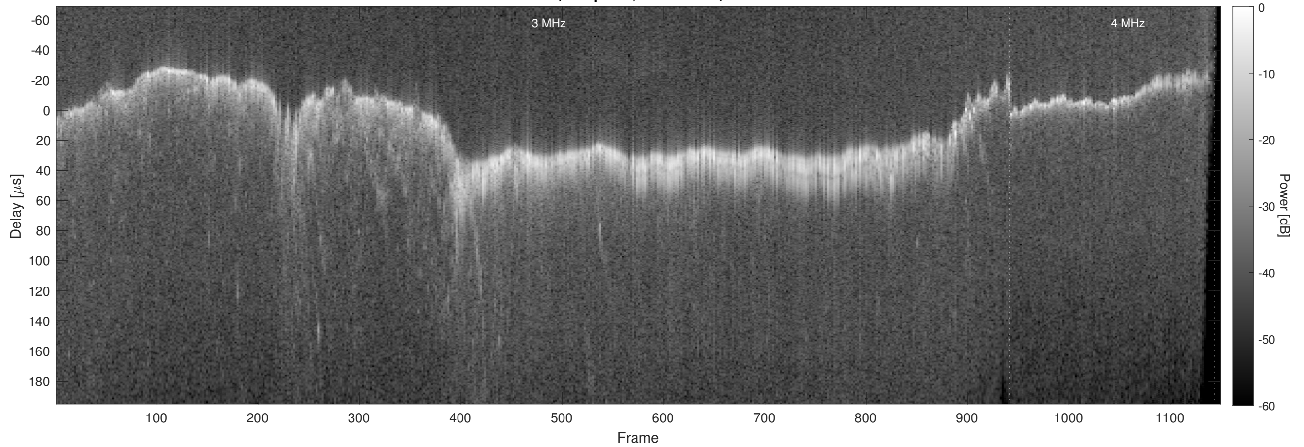
Orbit 10189, Chapman, No Window, Channel 2
