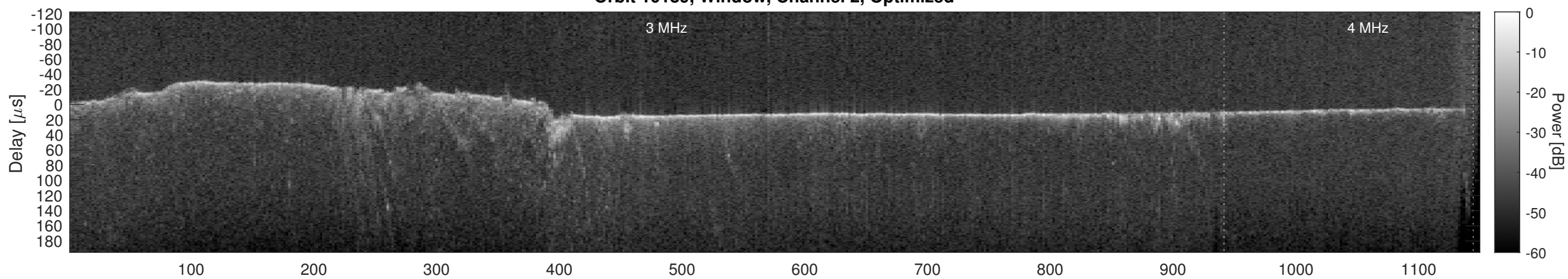
Orbit 10189, Cluttergram
