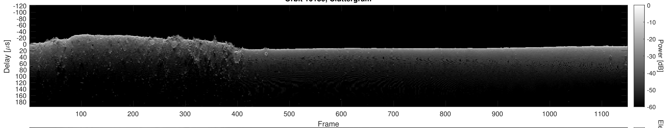
Orbit 10189, Cluttergram
