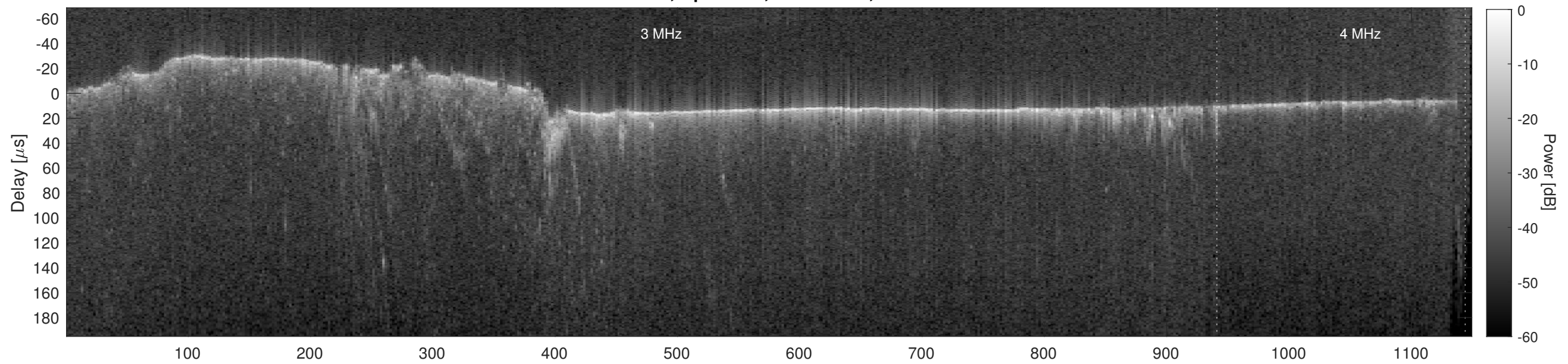
Orbit 10189, Cluttergram
