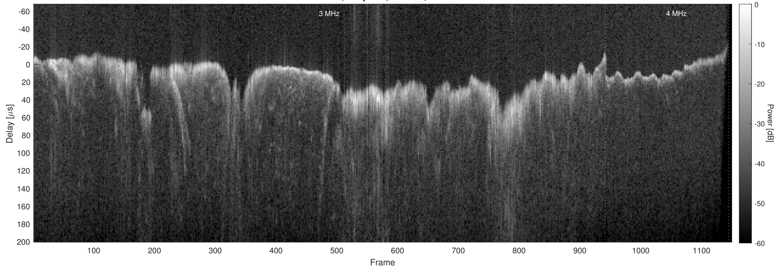
Orbit 10194, Chapman, Window, Channel 2
