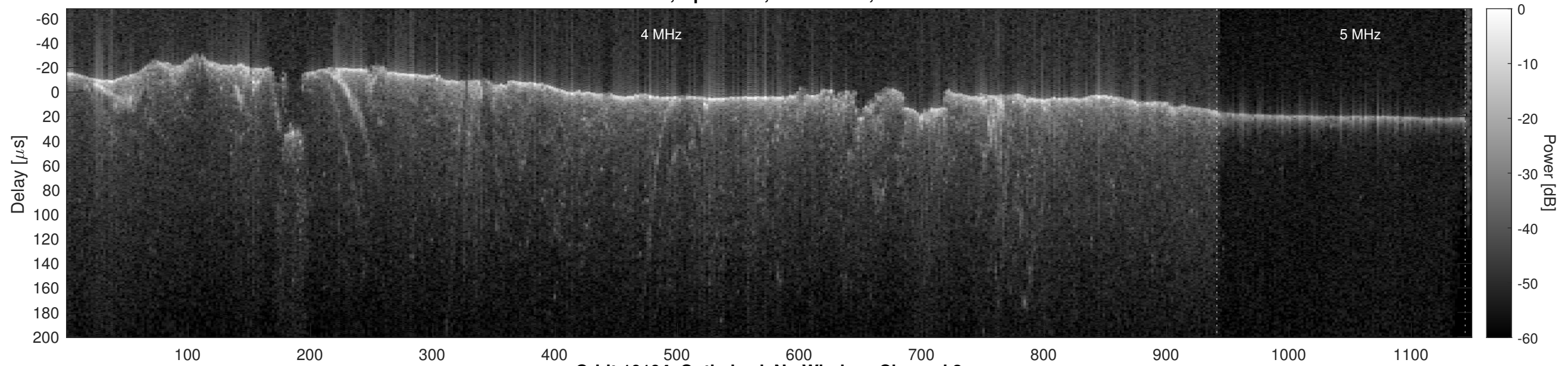
Orbit 10194, Optimized, No Window, Channel 2
