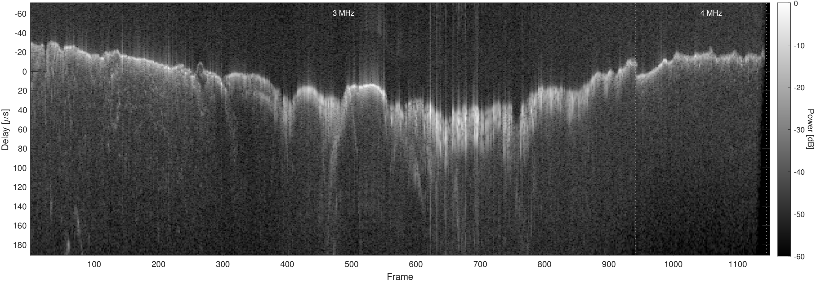
Orbit 10195, Chapman, No Window, Channel 2
