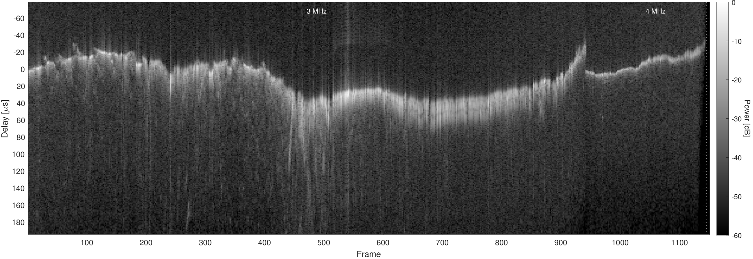
Orbit 10196, Chapman, No Window, Channel 2
