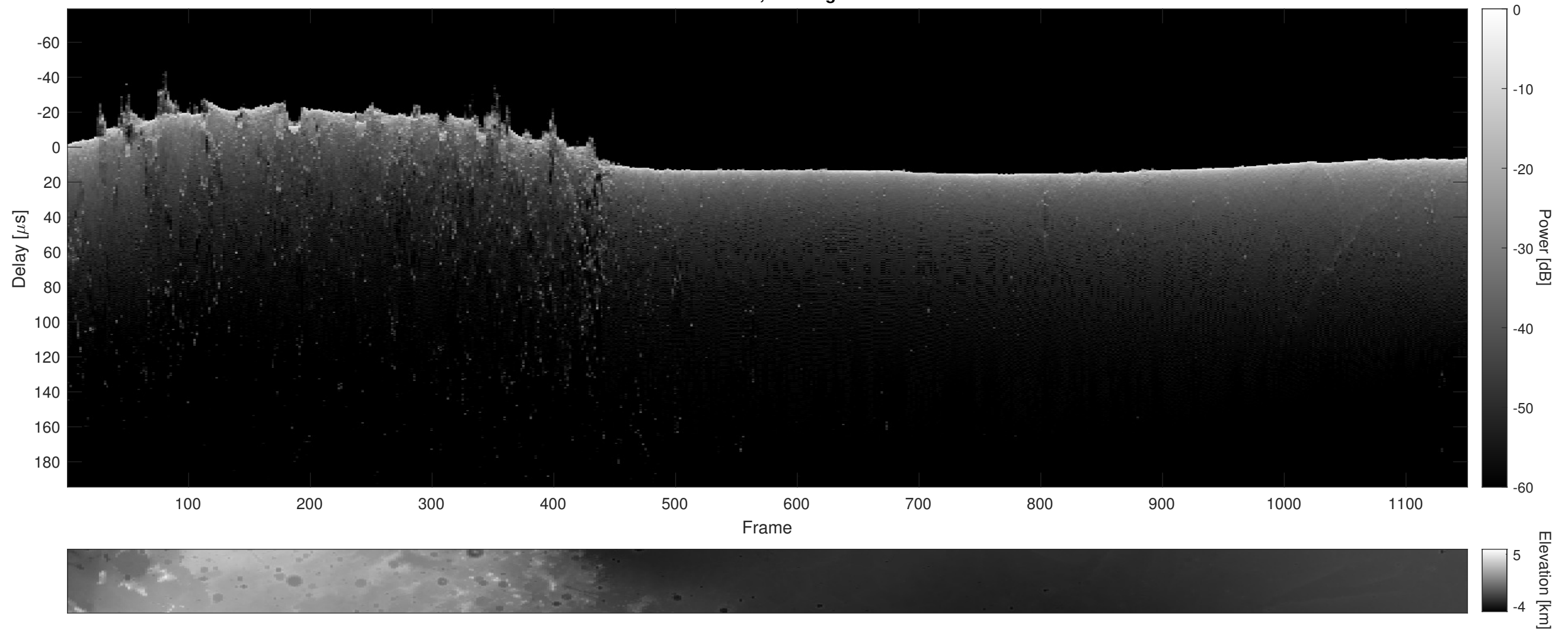
Orbit 10196, Cluttergram
