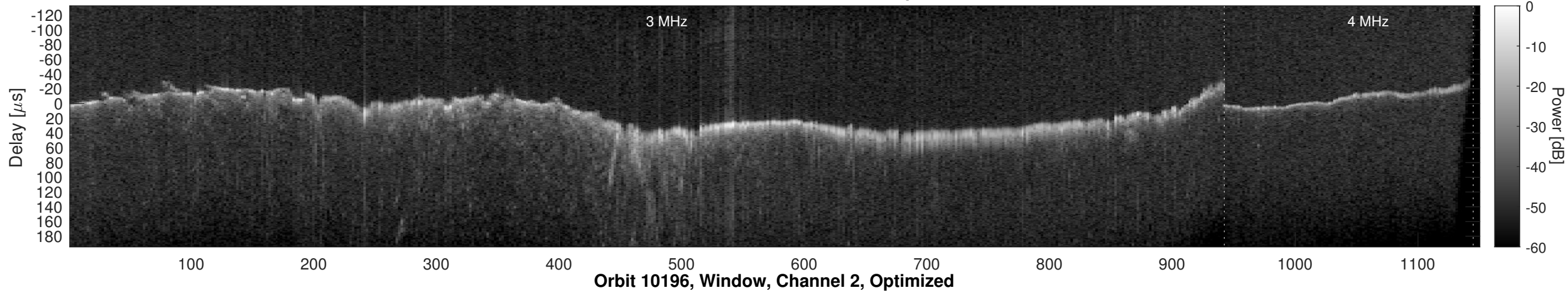
Orbit 10196, Window, Channel 2, Chapman
