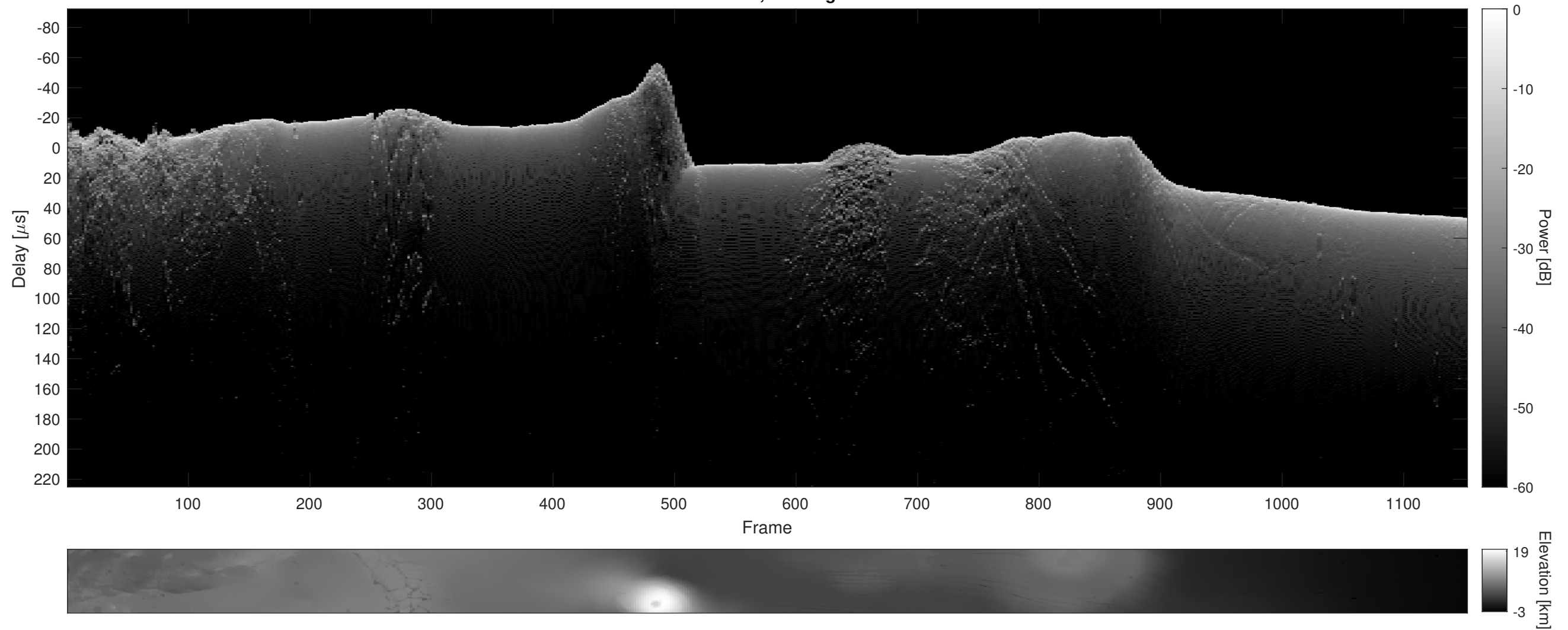
Orbit 10198, Cluttergram
