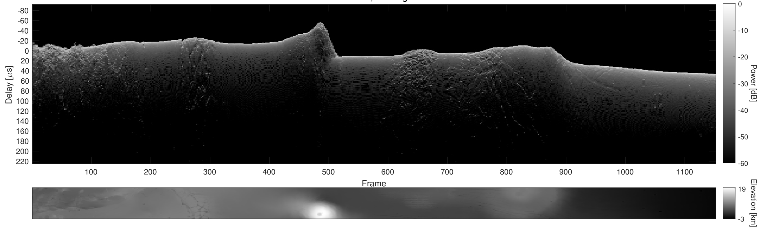
Orbit 10198, Cluttergram
