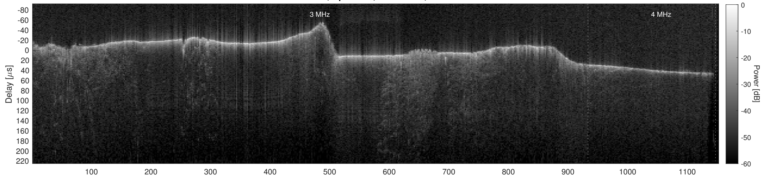
Orbit 10198, Cluttergram
