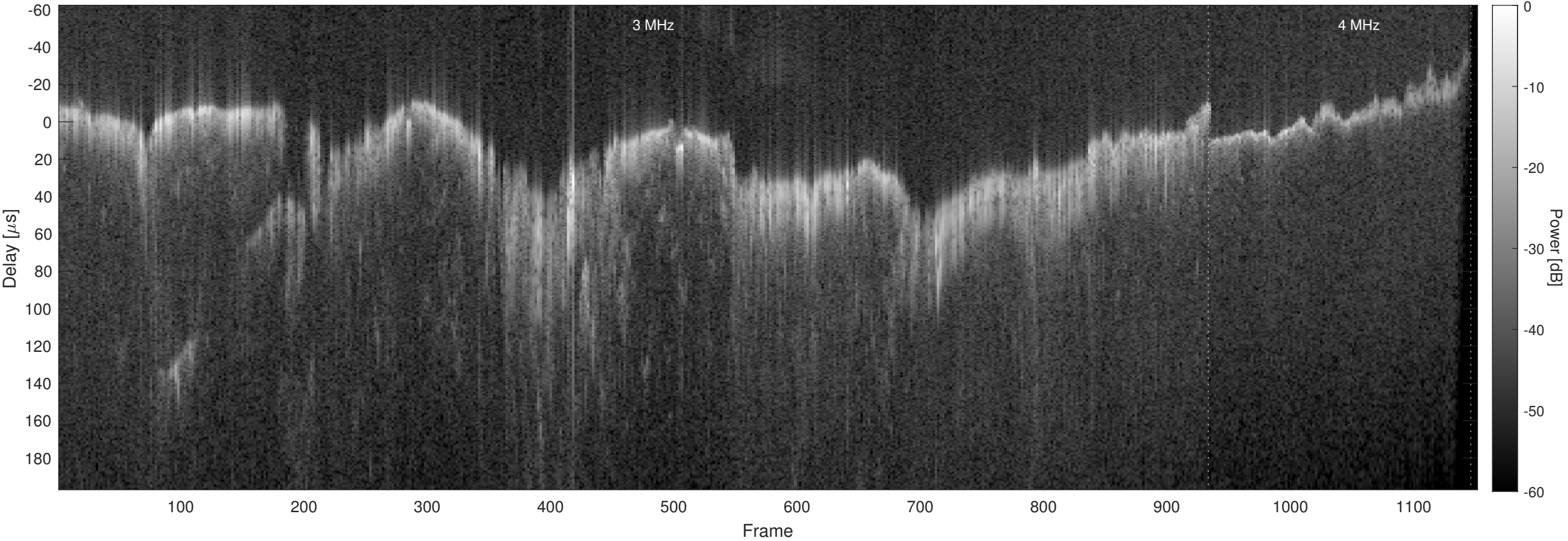
Orbit 10201, Chapman, No Window, Channel 2
