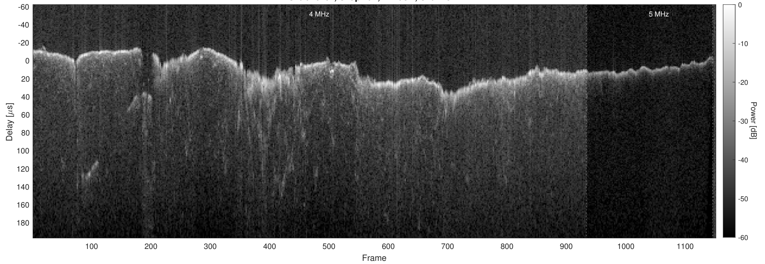
Orbit 10201, Chapman, Window, Channel 2
