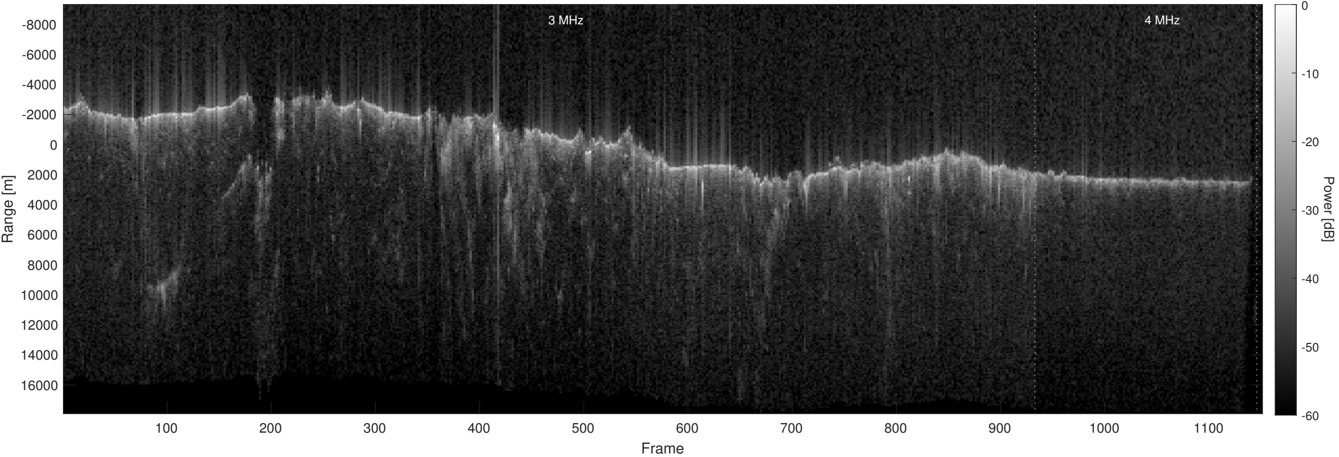
Orbit 10201, Optimized, No Window, Depth-Corrected, Channel 2
