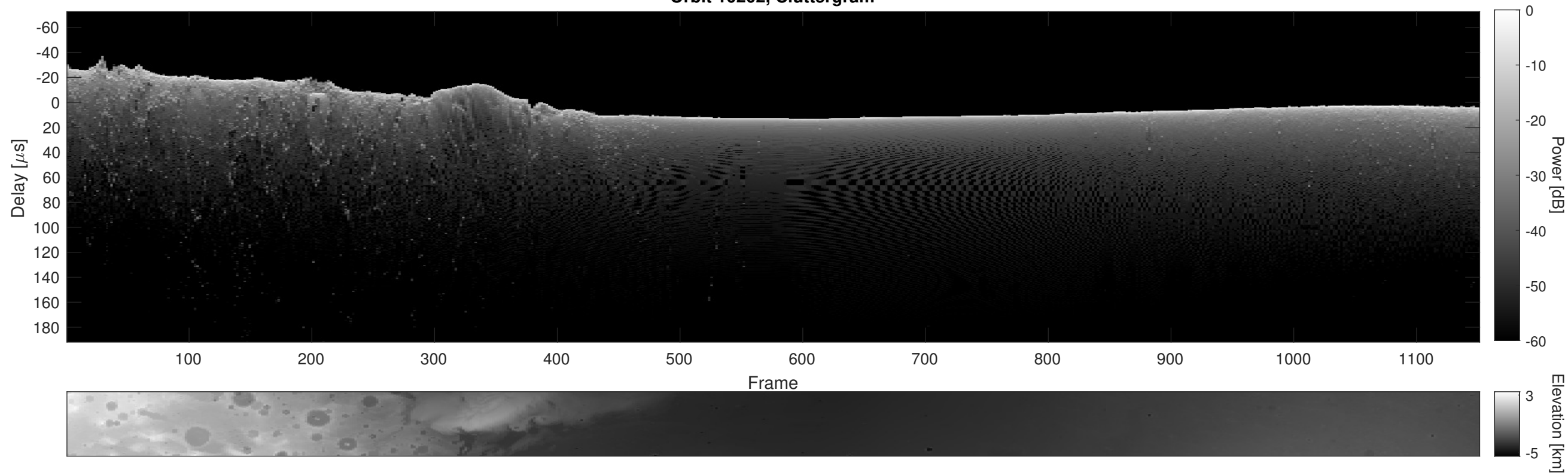
Orbit 10202, Cluttergram
