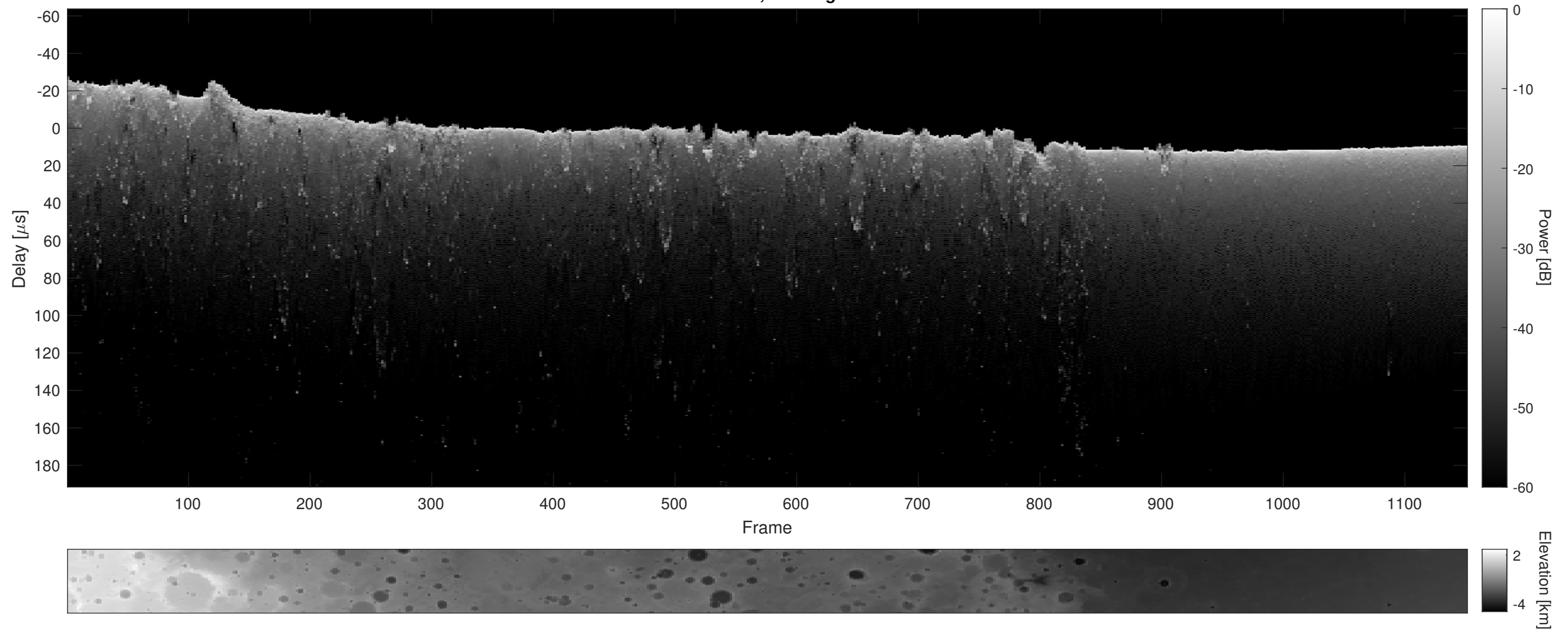
Orbit 10204, Cluttergram
