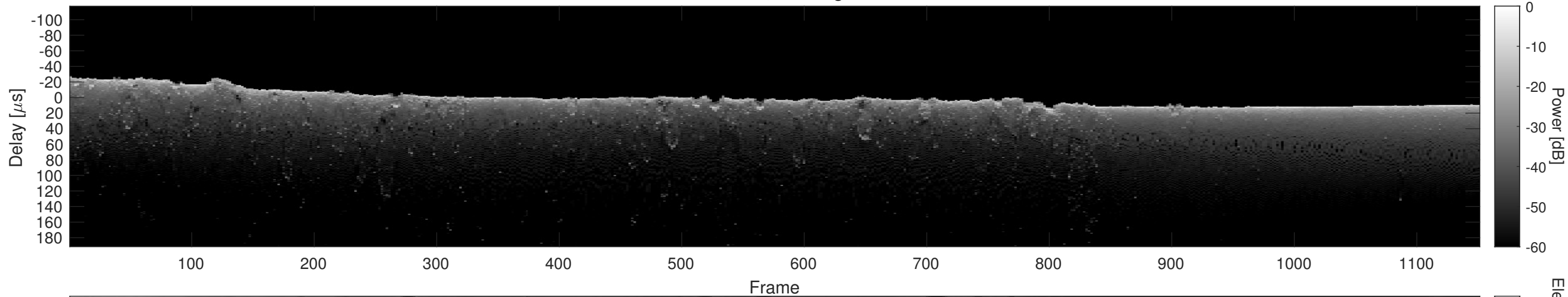
Orbit 10204, Cluttergram
