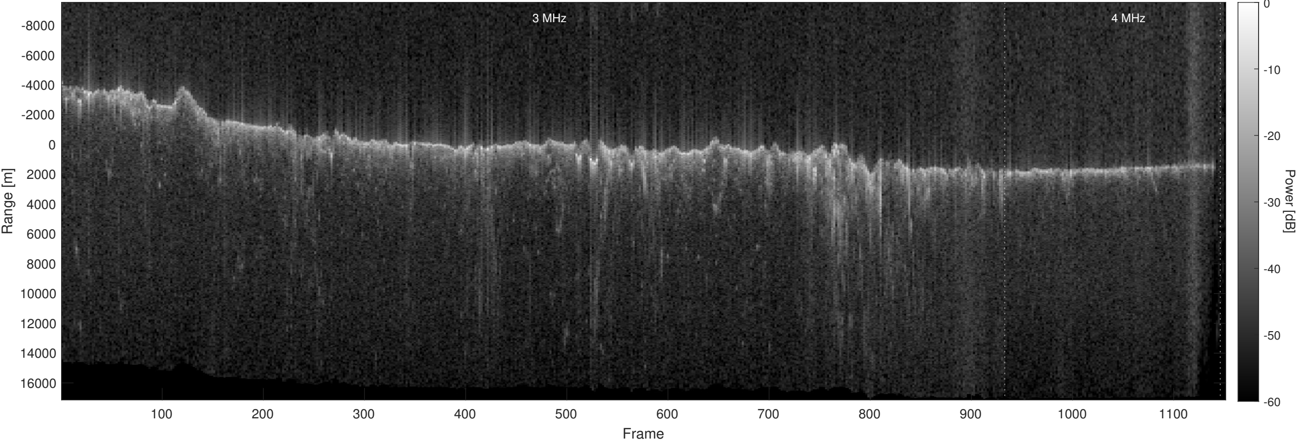
Orbit 10204, Optimized, No Window, Depth-Corrected, Channel 2
