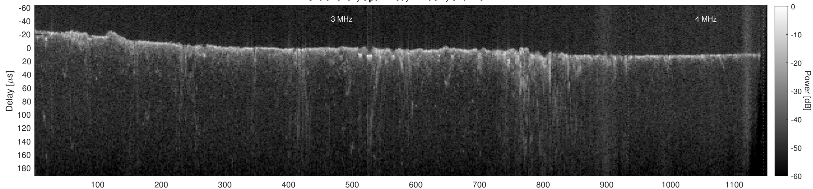
Orbit 10204, Cluttergram
