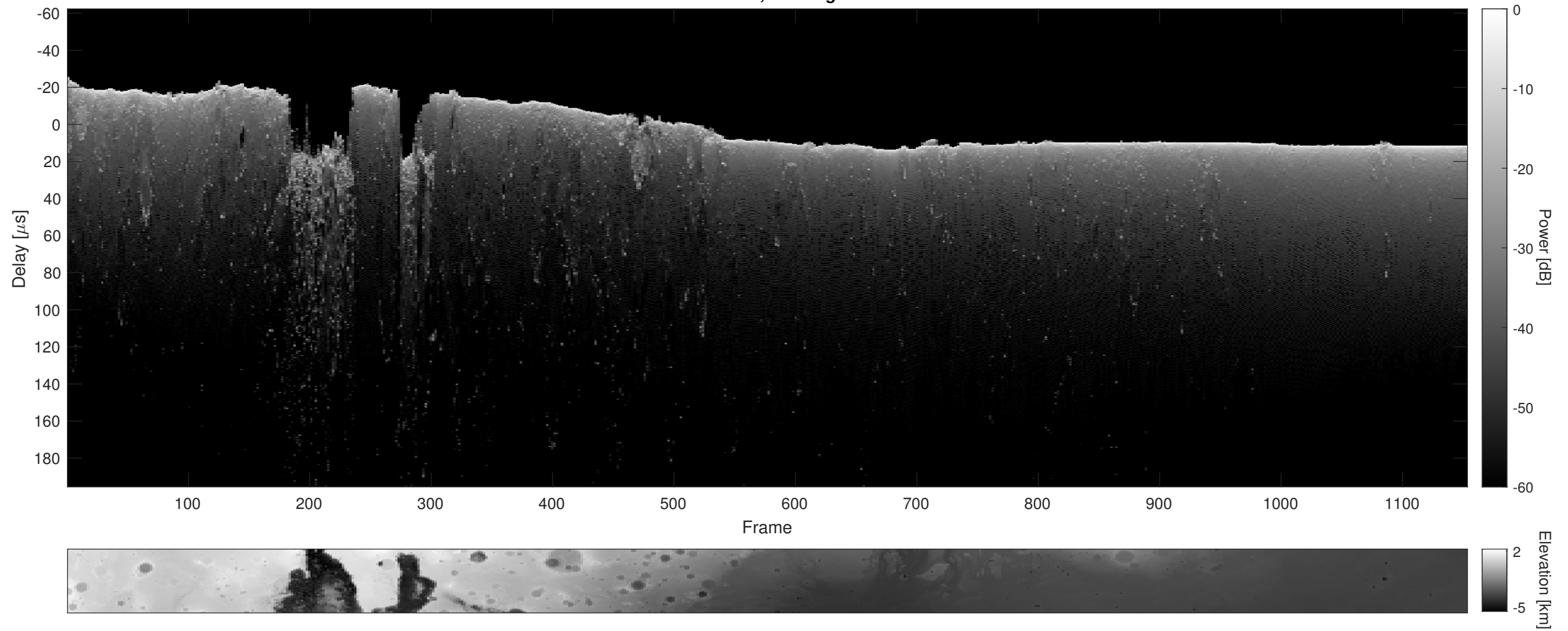
Orbit 10208, Cluttergram
