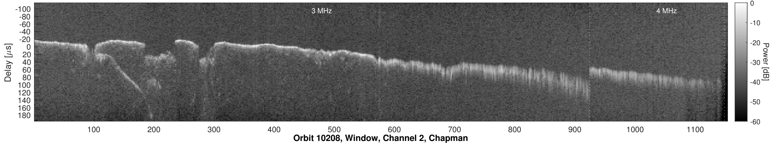
Orbit 10208, Window, Channel 2, Uncorrected
