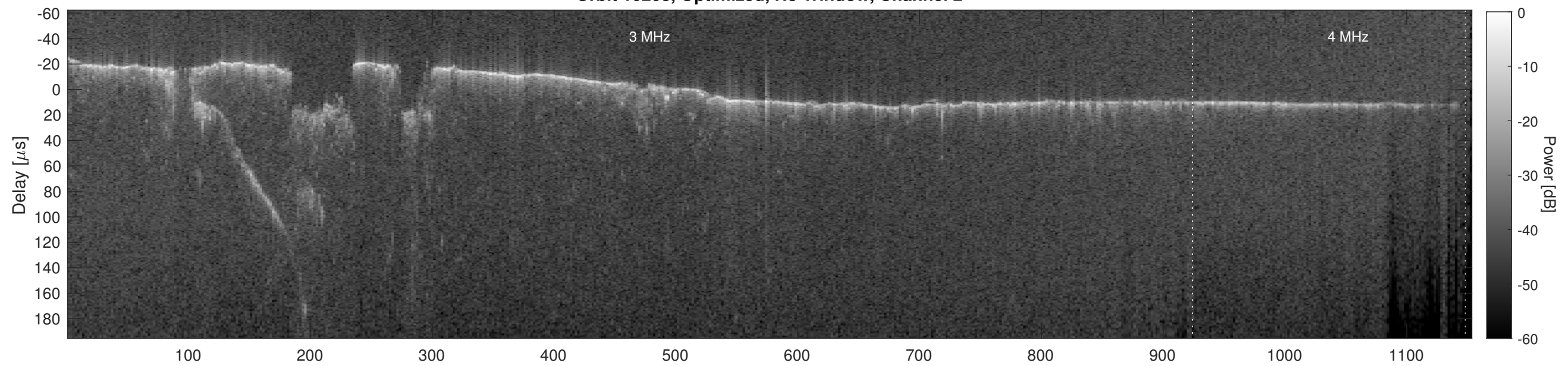
Orbit 10208, Cluttergram
