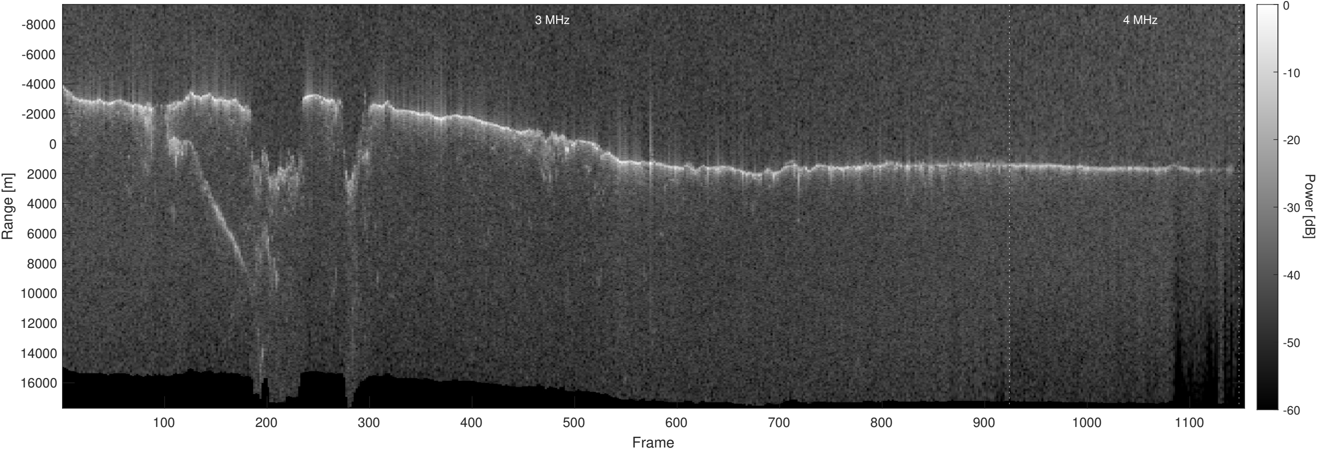
Orbit 10208, Optimized, No Window, Depth-Corrected, Channel 2
