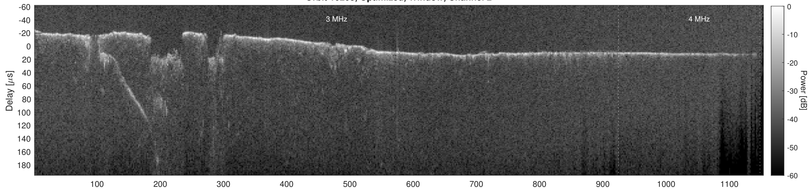
Orbit 10208, Cluttergram
