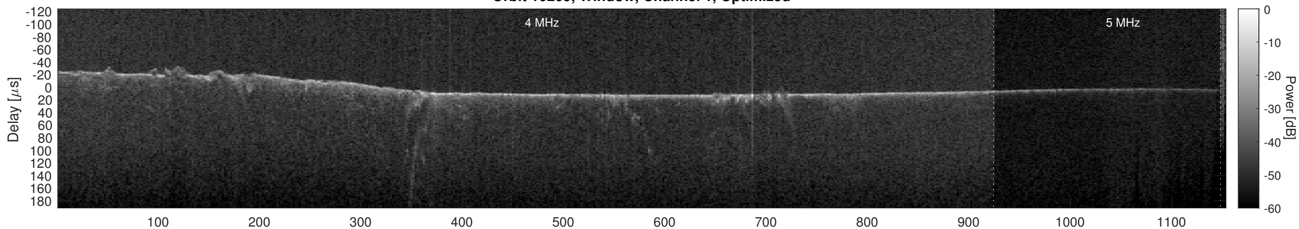
Orbit 10209, Cluttergram
